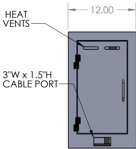
LEFT VIEW
