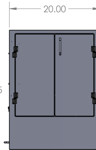
RIGHT VIEW
