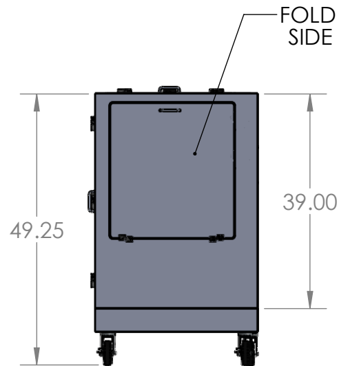
RIGHT VIEW
