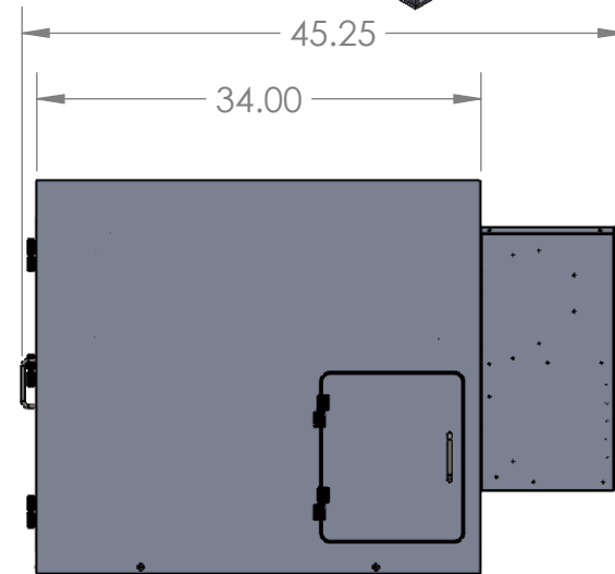
RIGHT VIEW
