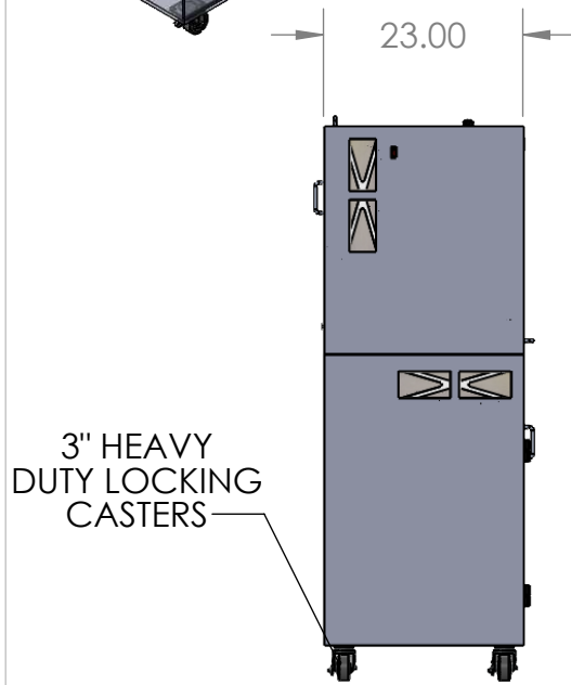
LEFT VIEW
