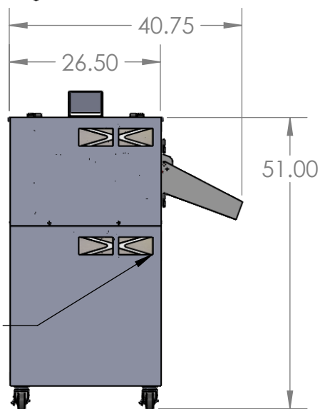
LEFT VIEW
