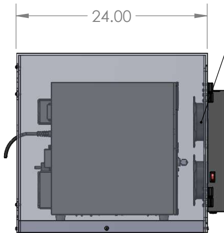
LEFT VIEW
