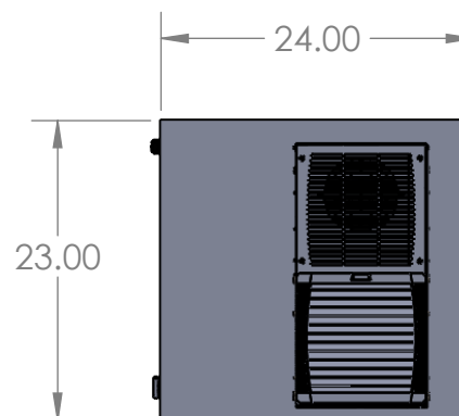
RIGHT VIEW
