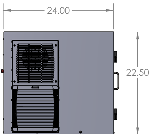
LEFT VIEW
