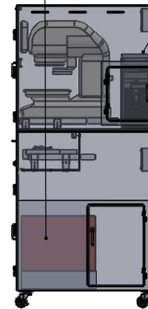
RIGHT VIEW
