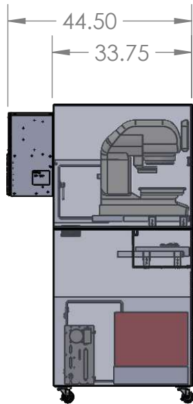
LEFT VIEW
