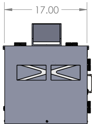
LEFT VIEW
