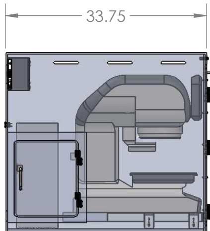
LEFT VIEW
