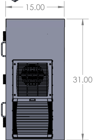
LEFT VIEW
