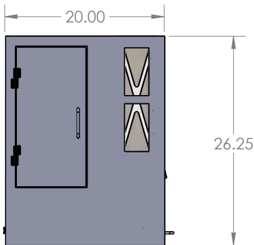
LEFT VIEW
