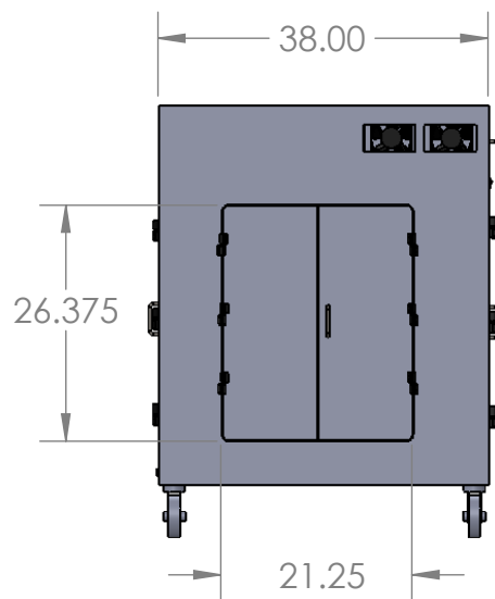
LEFT VIEW
