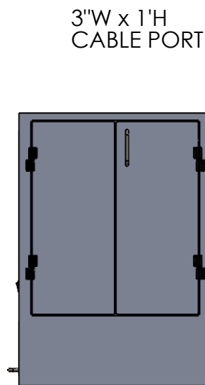
RIGHT VIEW
