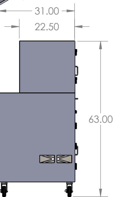
LEFT VIEW
