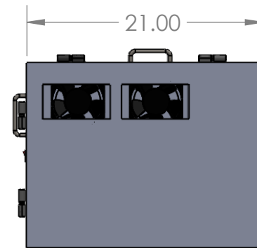
RIGHT VIEW
